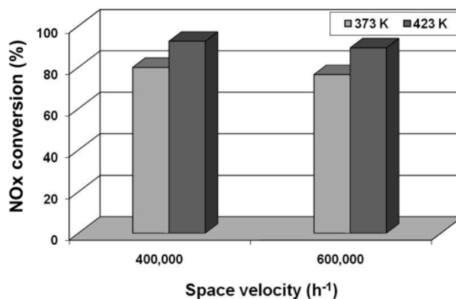
Fig. 3. NOx conversions over a MnOx-coated bag filters with a MnOx loading of 470 g/m 2 at 373 and 423 K. Reactants: 500 ppm NO and 500 ppm NH 3 in air.
